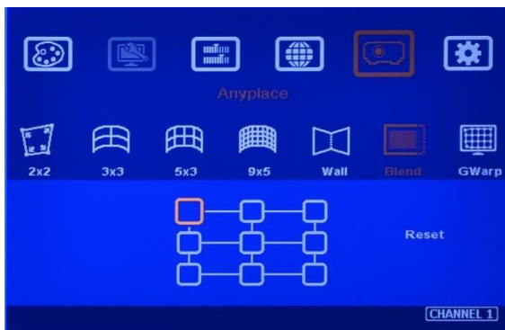
Nine regions black level uplift. Each region can set different RGB offset value.
